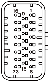
23 Pin Connector
